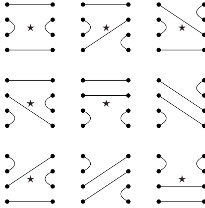
Figure 7: The upper \mathcal{D} -class of the subsemigroup \mathcal{U}_3 of \mathfrak{A}_4
