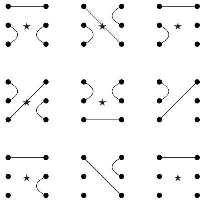
Figure 6: The upper \mathcal{D} -class of the subsemigroup \mathcal{U}_2 of P\mathcal{A}_3
